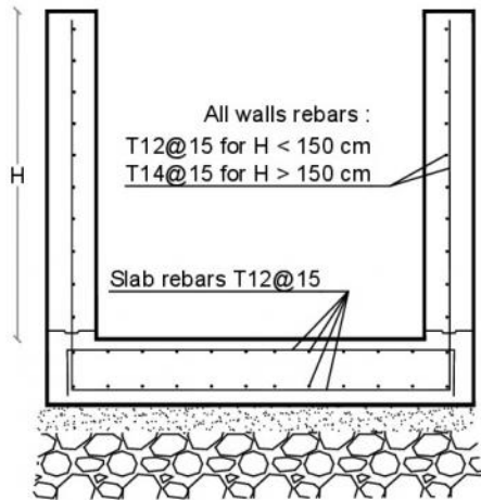
Canal Typical Cross Section
