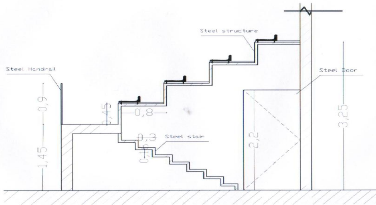
Section scale 1/50
