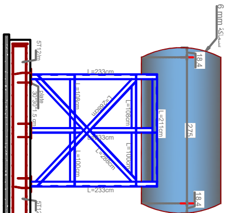
Section: D-D
