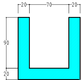
CONCRETE DITCH (U SHAPE)
