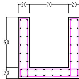
REINFORCEMENT DETAILS
