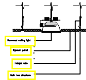
False Ceiling 1/20
