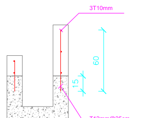
Steel detail
