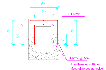
Steel detail
