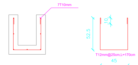
Steel detail
