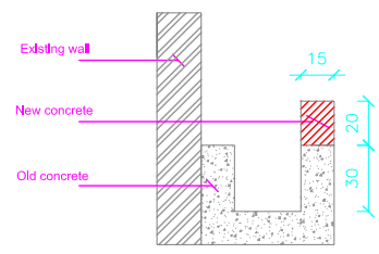
Modification for irrigation canal
