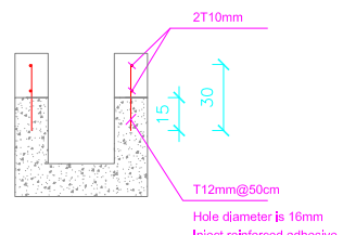
Steel detail
