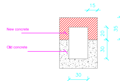
Modification for irrigation canal
