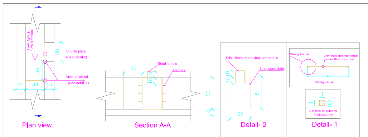
Sluice gate valve
