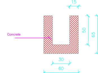
Modification for irrigation canal
