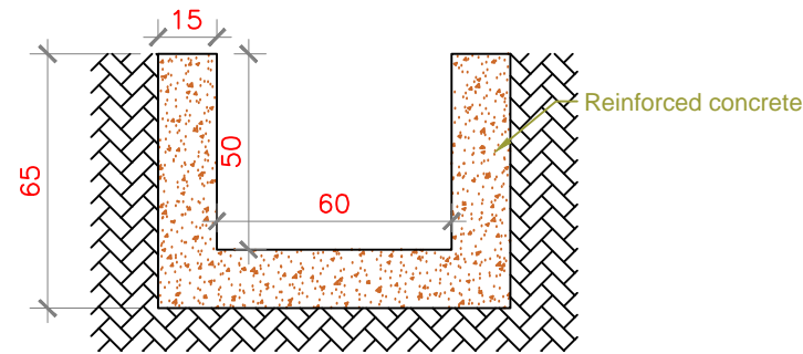
General Section Detail
