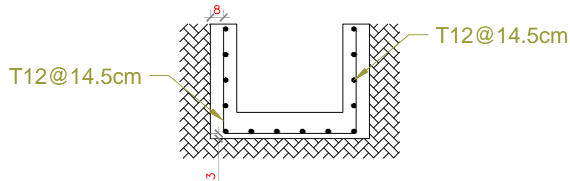
Reinforced Concrete section Detail
