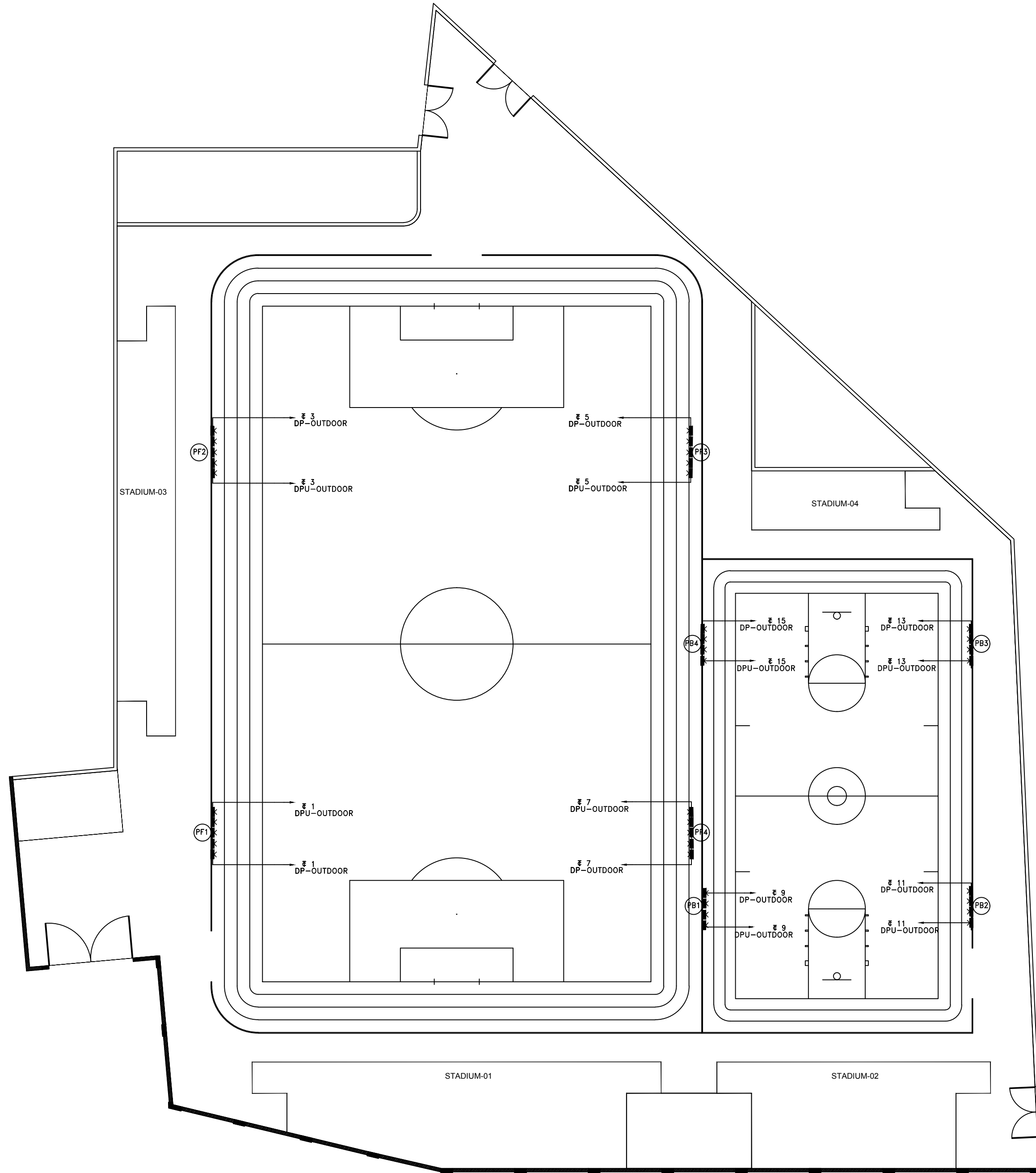
1 lighting poles E-101 Scale 1/200
